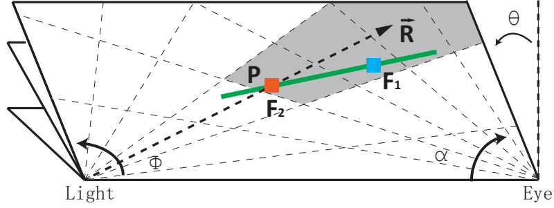
Figure 4. Incorrect shadowing in the epipolar coordinate system for VSVs. Gray voxels mean occluded. The voxel containing fragment F_1 is incorrectly shadowed by the voxel containing fragment F_2 .
