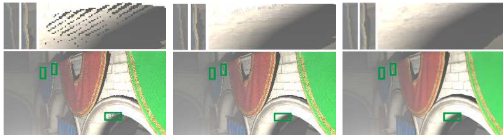
Figure 8. The scene is lit by an omni-directional light source through VSVs with a volume resolution of 1024 \times 1024 \times 512 . (left) Surface shadows are cast through VSVs with a constant bias. (center) Surface shadows are cast through VSVs with our adaptive bias. (right) Reference image. Surface shadows are cast with a 2D 8192 \times 8192 shadow map.
