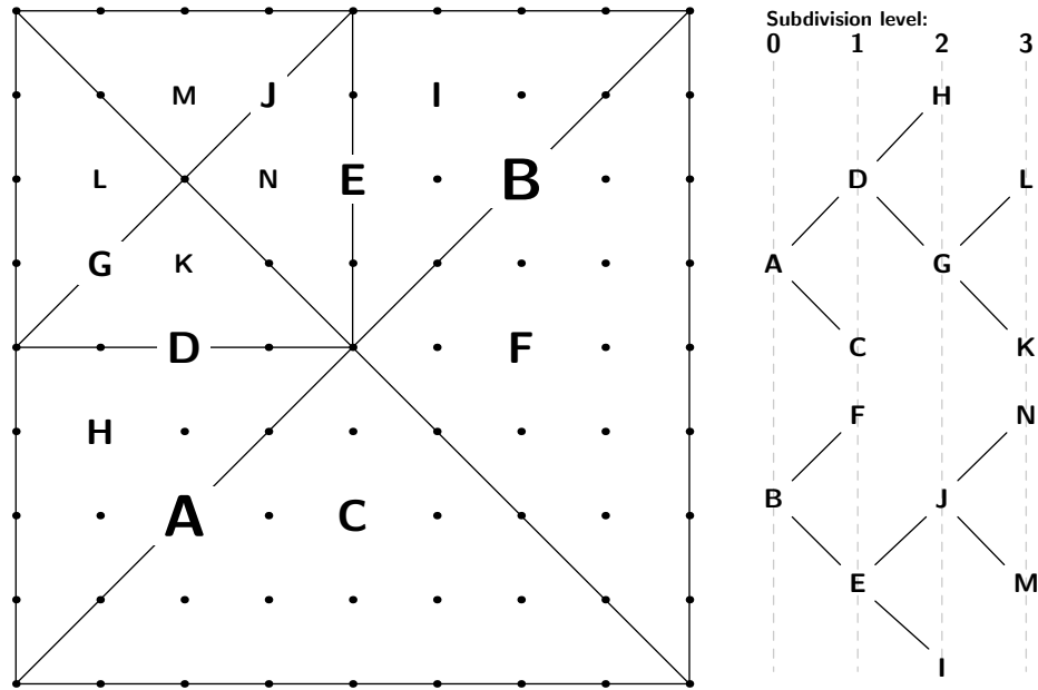
Figure 4. A triangulation of a 9 \times 9 heightmap as carried out by the ROAM tessellation algorithm. The triangulation begins with two triangles, marked A and B above, which span the entire heightmap and proceeds with splitting operations, which yield new pairs of triangles. The process therefore creates a binary tree of triangles, with the important property that all triangles within a subtree are nested within the triangle at which the subtree is rooted.
