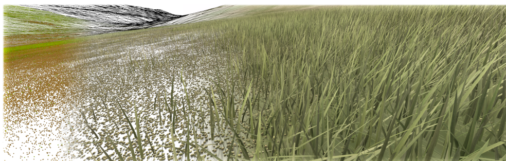
Figure 1. Two kinds of objects scattered over a large terrain area. One is regular grass, which covers areas of the terrain that appear green, while the other consists of simple gravel-like particles which cover brown areas.
