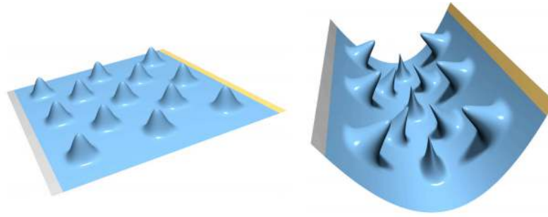
Figure 13. A plane using displacement mapping for bumps (left). When the plane bends (right), the volumetric space near the bend is compressed, resulting in the nearby bumps getting distorted. Figure from [Botsch and Sorkine 2008].
