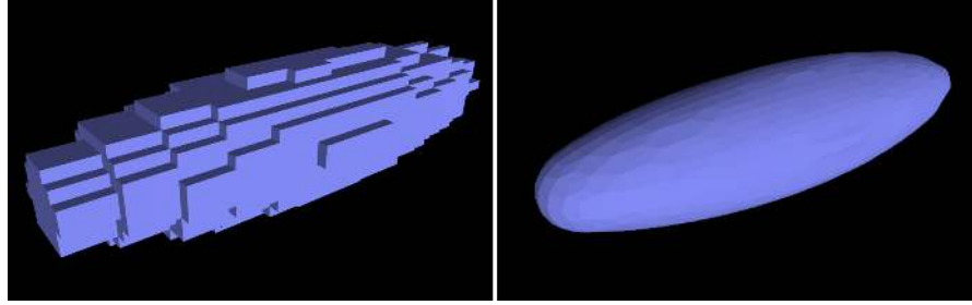
Figure 10. SurfaceNets handles smoothing of non-cubic voxels well. Left: a cuberille surface of an ellipsoid with voxel size 1\text{ mm} \times 1\text{ mm} \times 4\text{ mm} . Right the SurfaceNet generated for this model.
