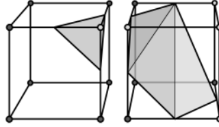
Figure 2. Marching Cubes surface patches for two different cells. The surface intersects a cell if at least one of the 8 corner values is different from the others (Here, light/dark corners are inside/outside respectively). For each cell intersecting the surface, a surface patch is constructed which lies entirely inside the cell. Surface vertices are constrained to lie on cell edges.
