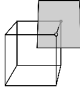
Figure 3. Dual contouring methods place surface vertices inside cells. Surface quadrilaterals are constructed by connecting vertices in neighboring cells that share an edge intersected by the iso-surface (e.g., here a surface quadrilateral is constructed for the top-right edge by connecting the vertex in this cell to the vertices of its right, top, and top-right neighbor cells). Surface vertices can be moved around inside the cell to improve surface quality.
