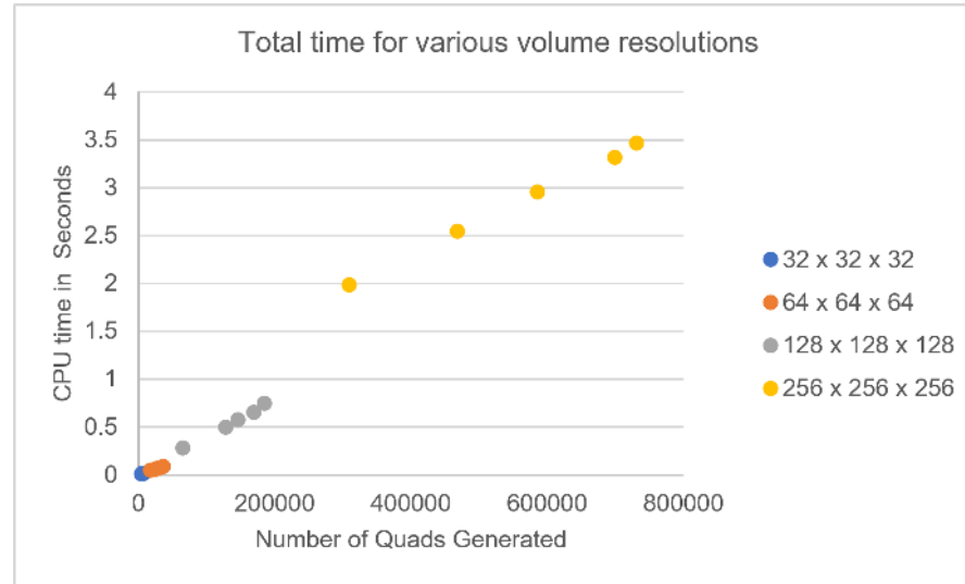
Figure 13. The total time required to generate the SurfaceNet, fair the surface, and export geometry for rendering varies approximately linearly with the number of quadrilaterals in the surface mesh, which depends on the dimensions of the 3D volume containing the multi-label data and the complexity of the surface in the data. In this test, the complexity of the surface was controlled by the number of randomly generated spheres composed to generate the labeled data.
