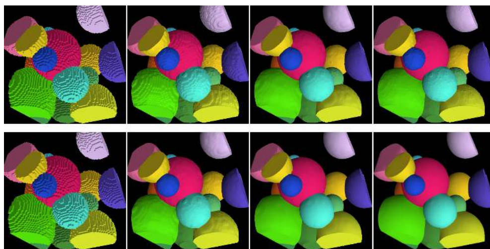
Figure 9. The effect of surface fairing parameters on smoothness and accuracy. Vertices are constrained to lie within 0.5 mm and 1 mm of the center of the 1 \text{ mm} \times 1 \text{ mm} \times 1 \text{ mm} voxels for the top and bottom rows, respectively. From left to right: no smoothing, too few smoothing iterations, optimal iterations, too many iterations for the given accuracy.
