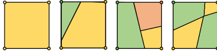
Figure 4. Face types from left-to-right: SolidFace, SurfaceFace, JunctionFace (2 JunctionFace examples shown). JunctionFace includes faces intersected by more than two materials and faces intersected by two materials where vertices of the same material are located on diagonally opposite corners (far right).
