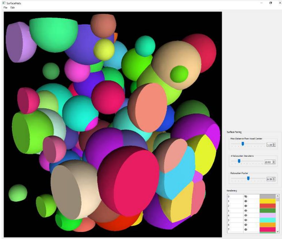
Figure 7. A screen shot of a simple application for testing and demonstrating the proposed method. The model here was generated from 100 spheres with random center positions and radii inside a 256 \times 256 \times 256 volume. Sliders on the right control panel are used to adjust surface fairing parameters. The SurfaceNet is rendered using flat shading for better evaluation of surface smoothness.
