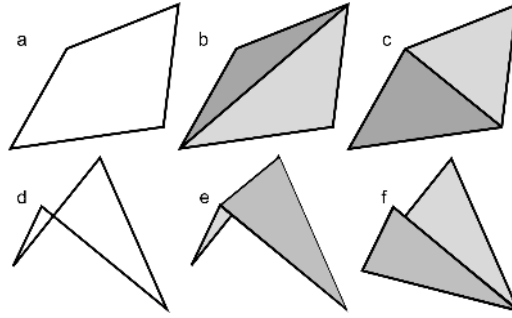
Figure 6. Quadrilaterals (a, d) can be partitioned into two different triangle patterns (b, c and e, f). When the quadrilateral is non-planar (d), the choice of partitioning can impact local shape.
